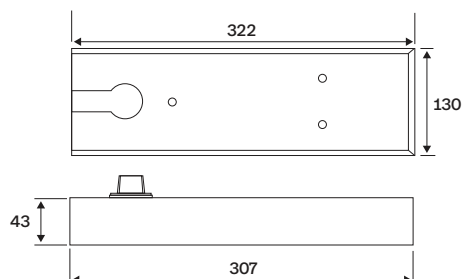
Dimension
